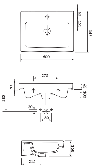
K114-006 UMYWALKA MEBLOWA CREA 60 CREA 80 FURNITURE WASHBASIN
