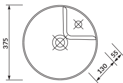
K114-002 UMYWALKA WPUSZCZANA W BLAT CREA 38 CREA 38 LET IN COUNTERTOP WASHBASIN ROUND
