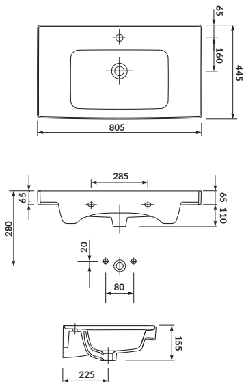
K114-017 UMYWALKA MEBLOWA CREA 80 CREA 80 FURNITURE WASHBASIN
